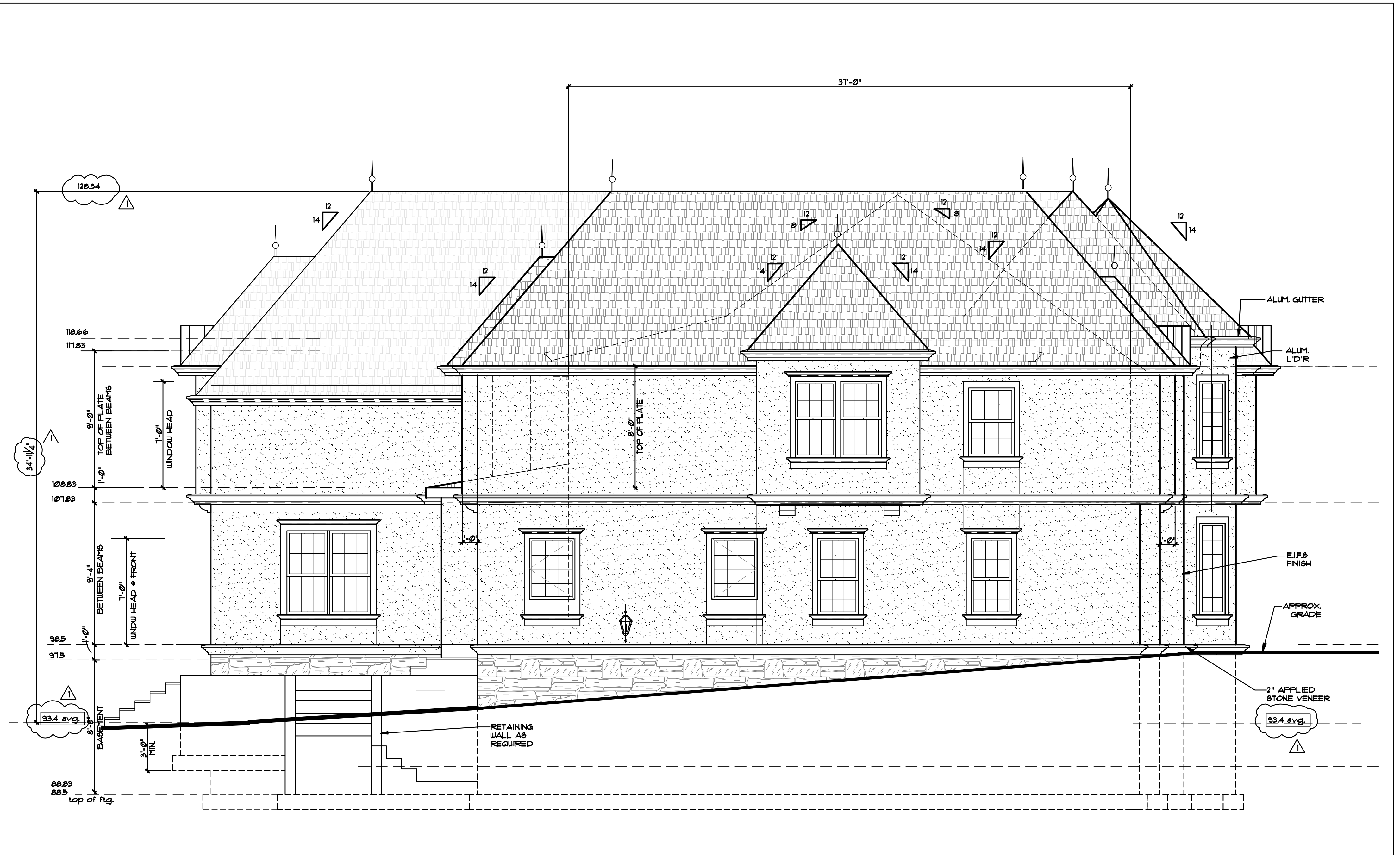
LEFT SIDE ELEVATION SCALE : 1/4" = 1'-0"
