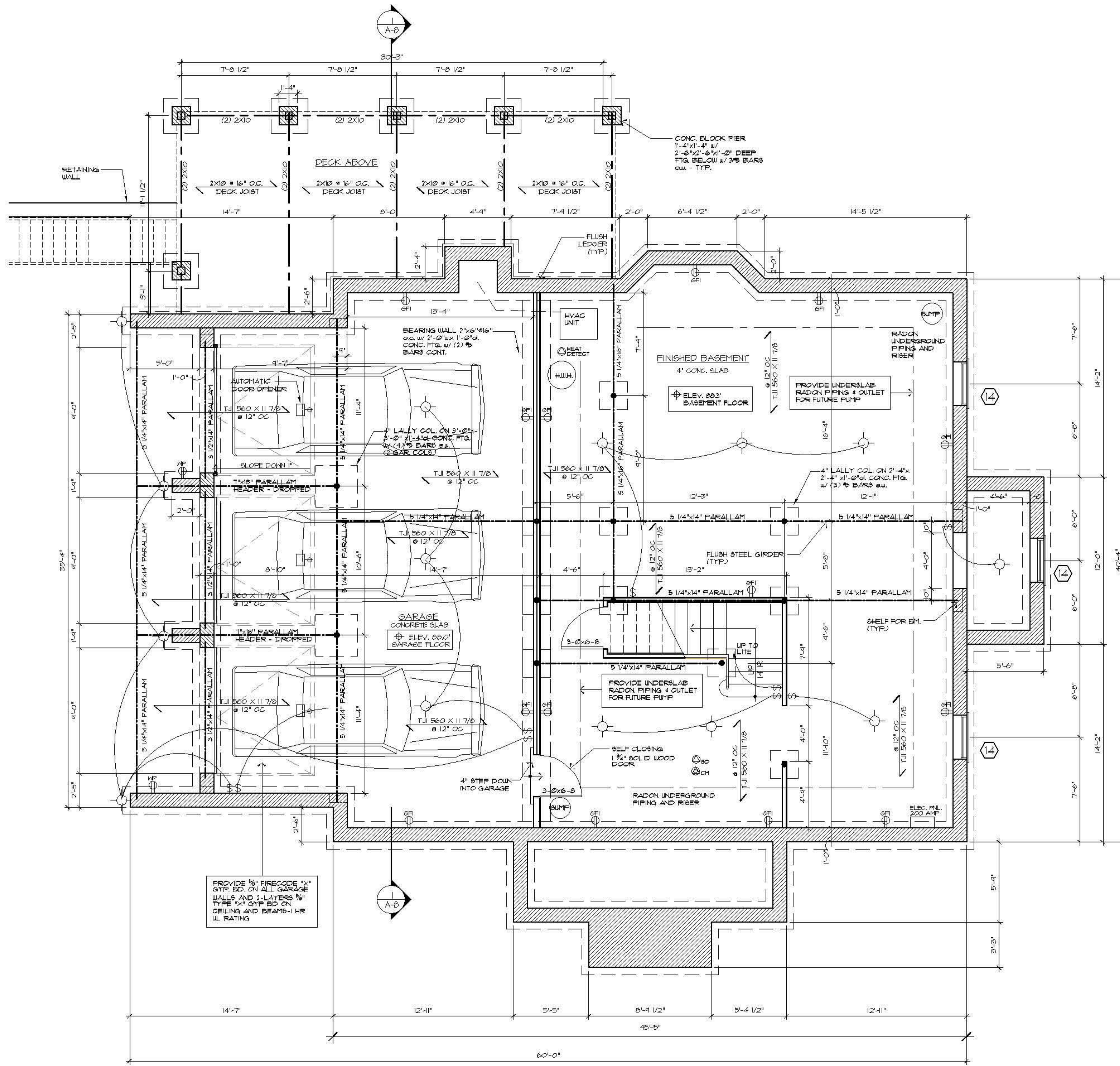
BASEMENT FLOOR PLAN SCALE: 1/4"=1'-0"
