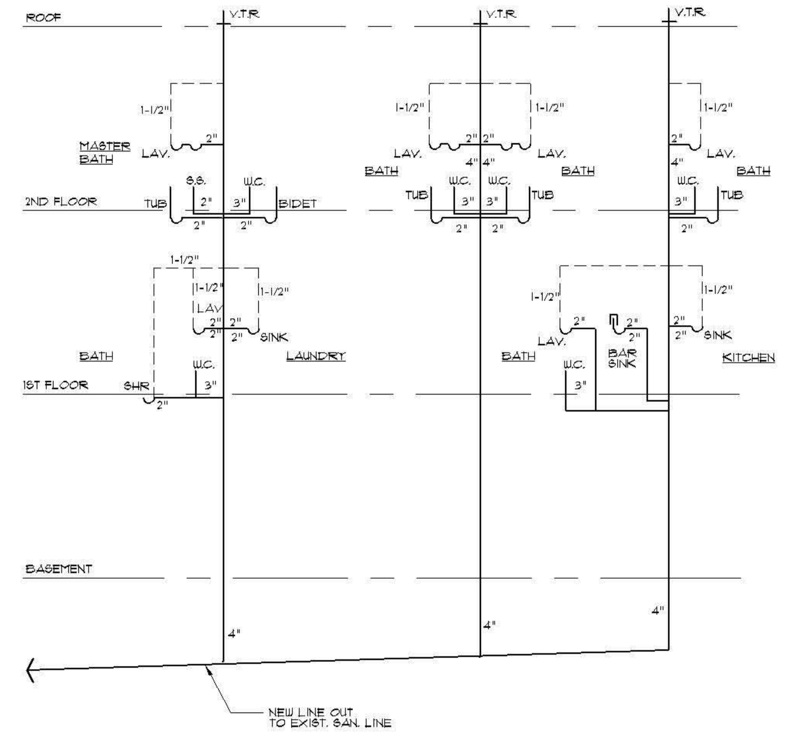
PLUMBING RISER DIAGRAM NO SCALE
