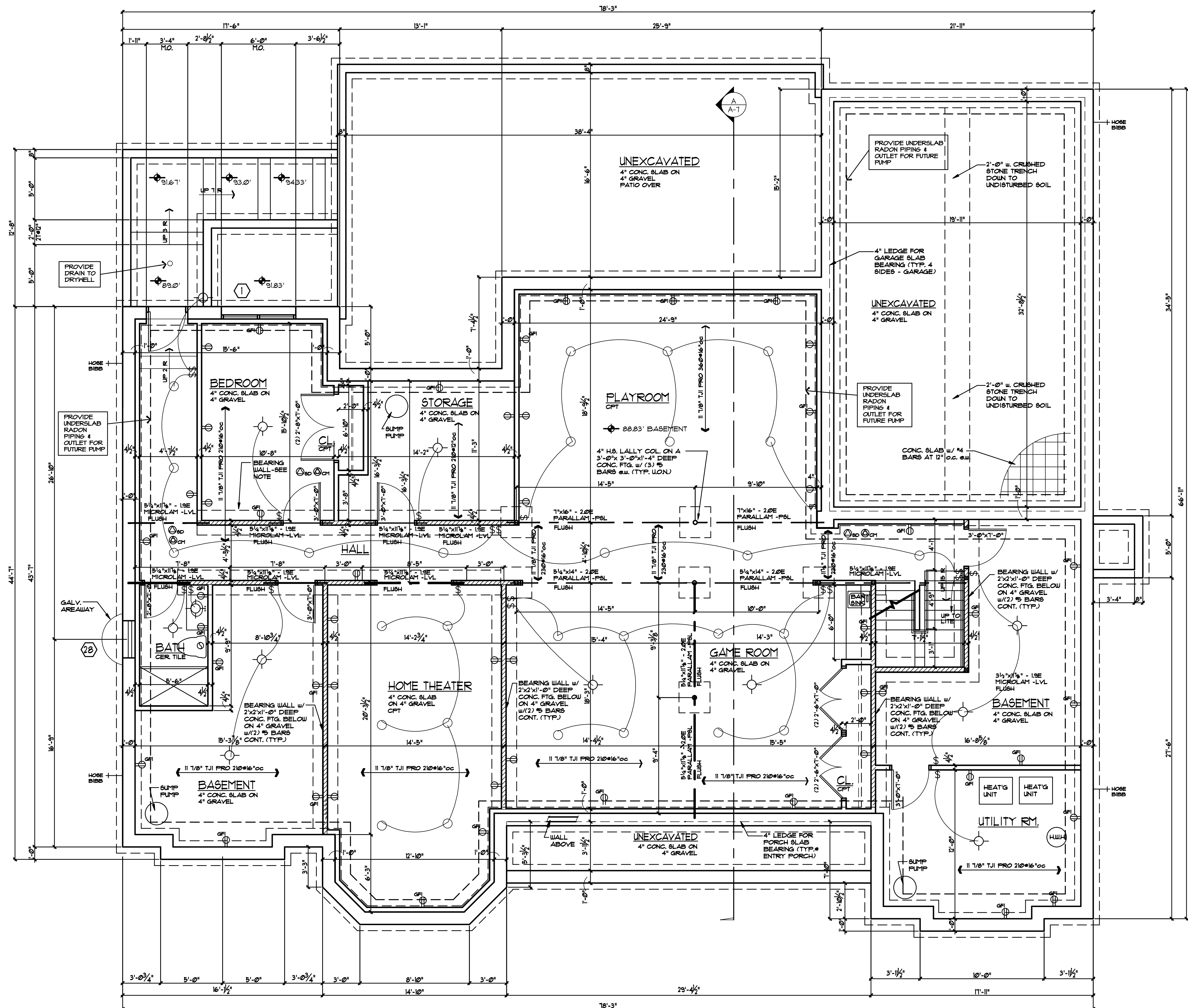
BASEMENT PLAN SCALE : 1/4" = 1'-0"
