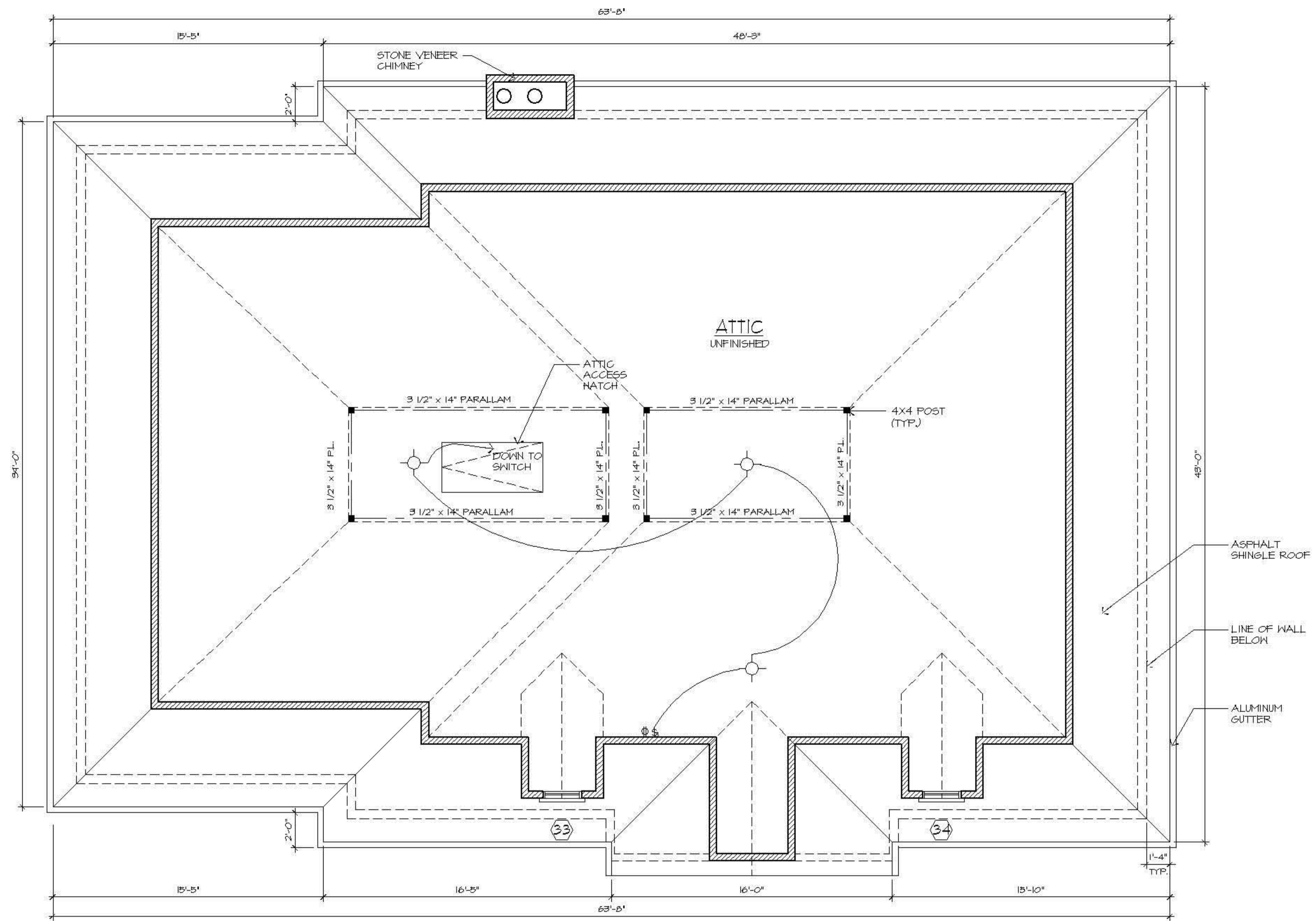
ATTIC FLOOR PLAN SCALE: 1/4"=1'-0"
