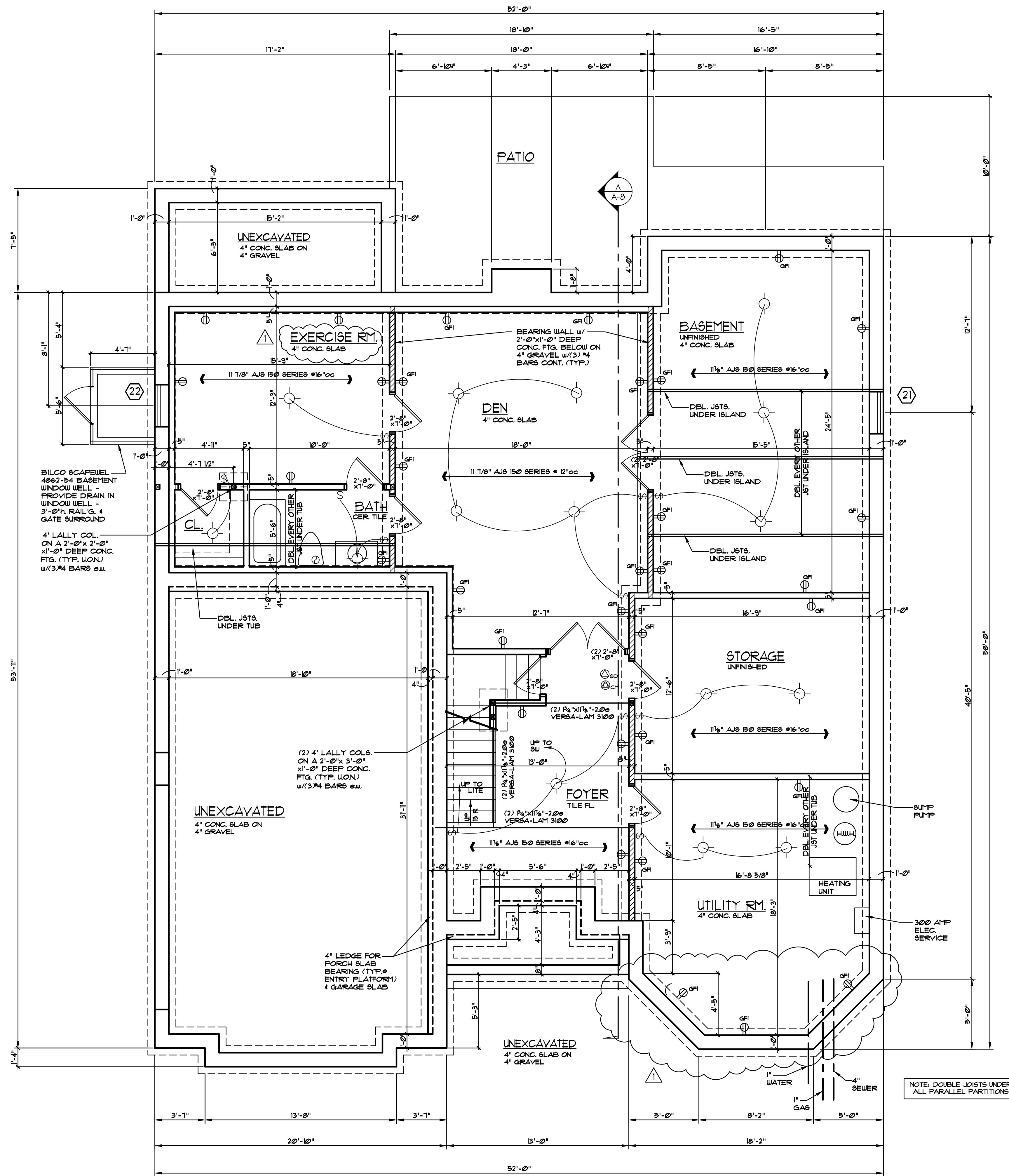
BASEMENT PLAN SCALE : 1/4" = 1'-0"
