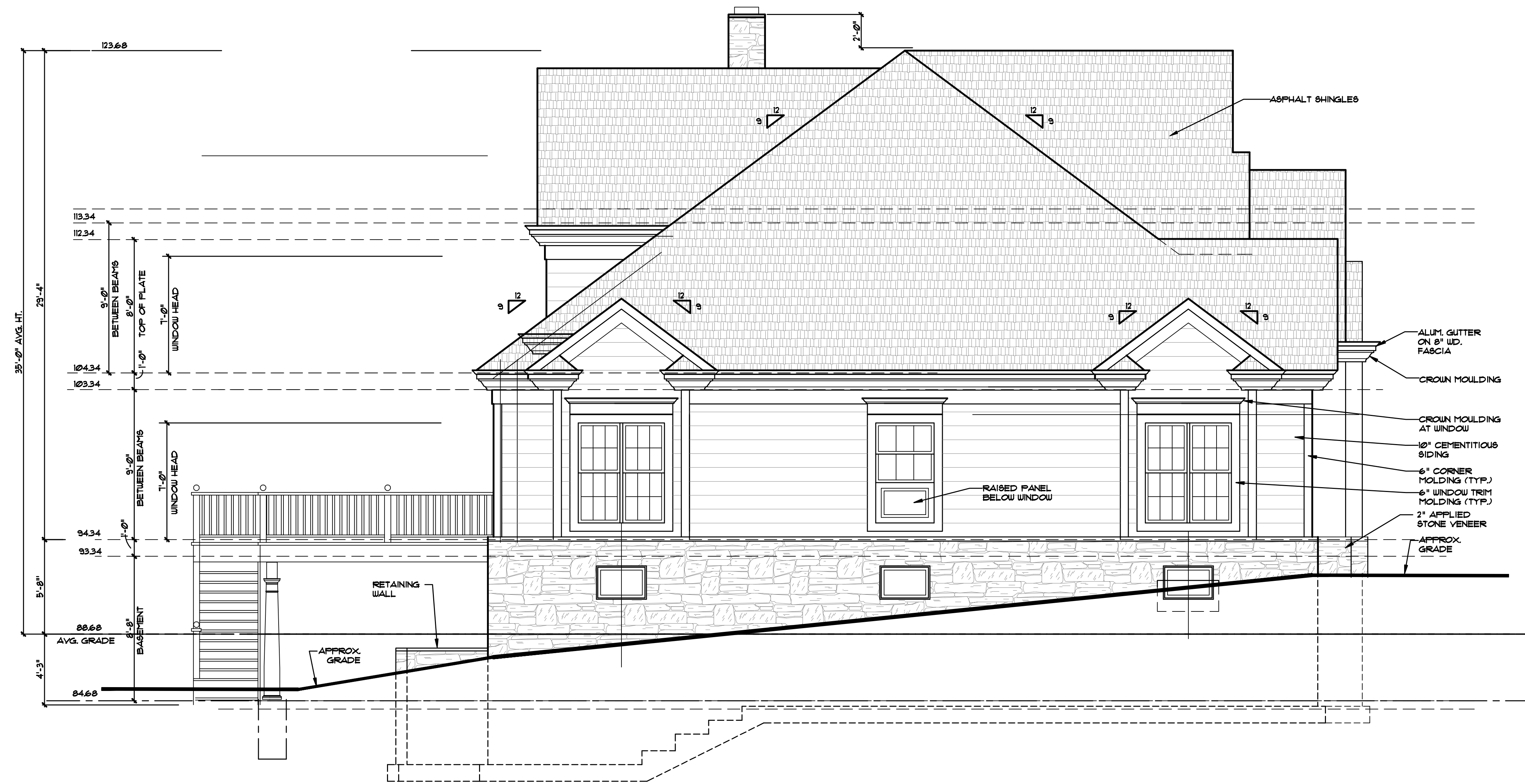
LEFT SIDE ELEVATION SCALE : 1/4" = 1'-0"
