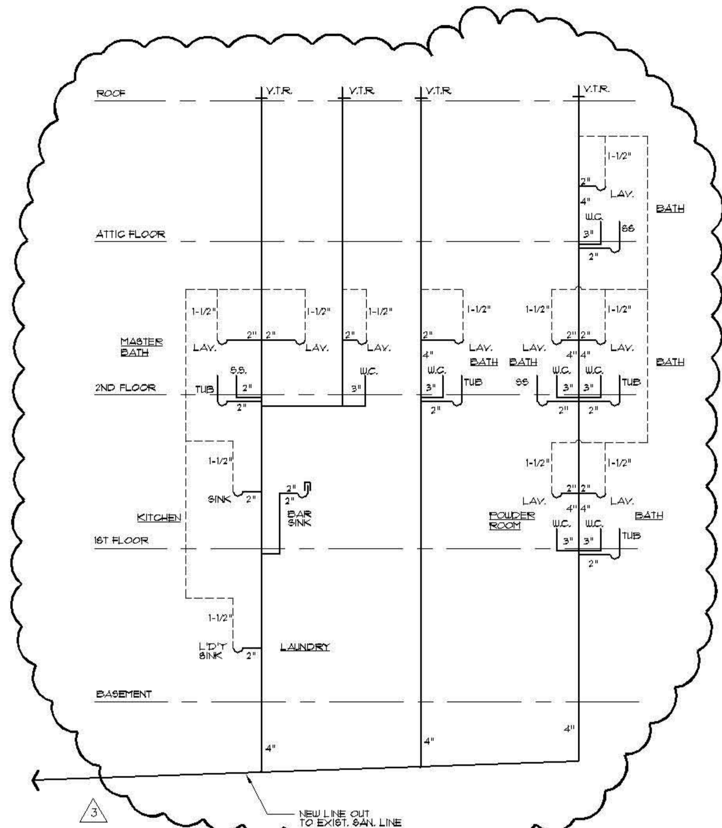
PLUMBING RISER DIAGRAM NOT TO SCALE
