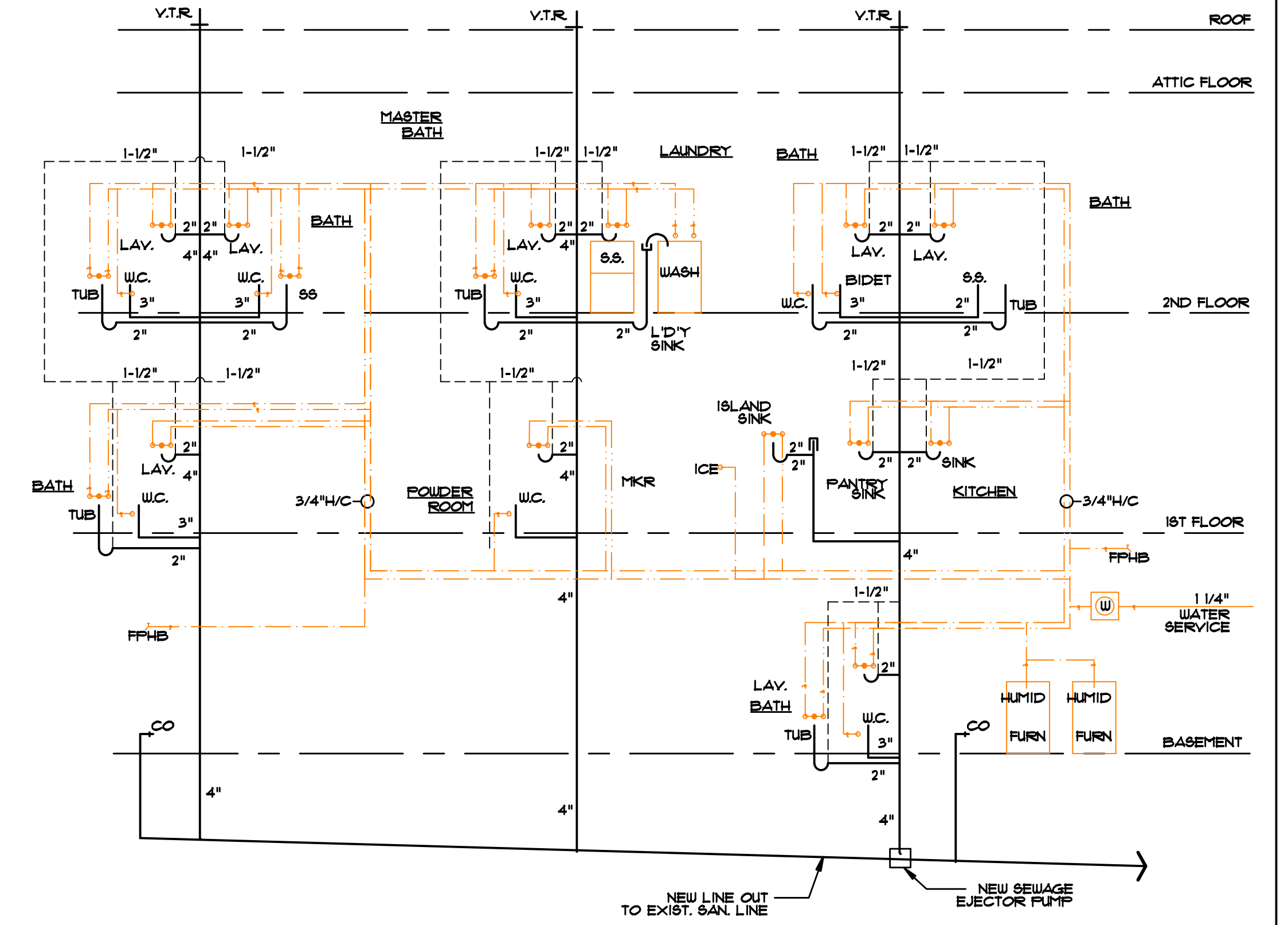
WATER RISER DIAGRAM NOT TO SCALE
