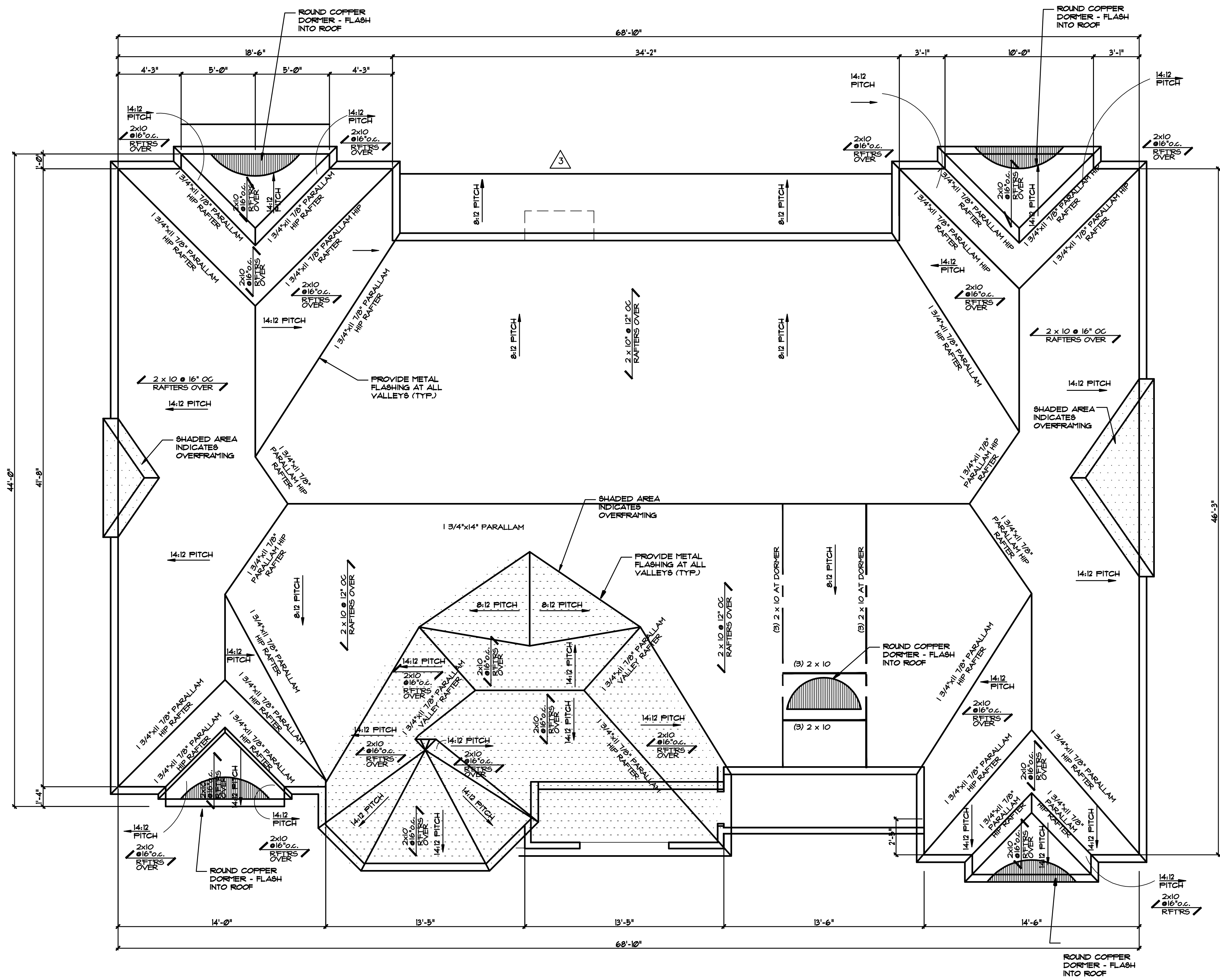
ROOF PLAN SCALE: 1/4" = 1'-0"
