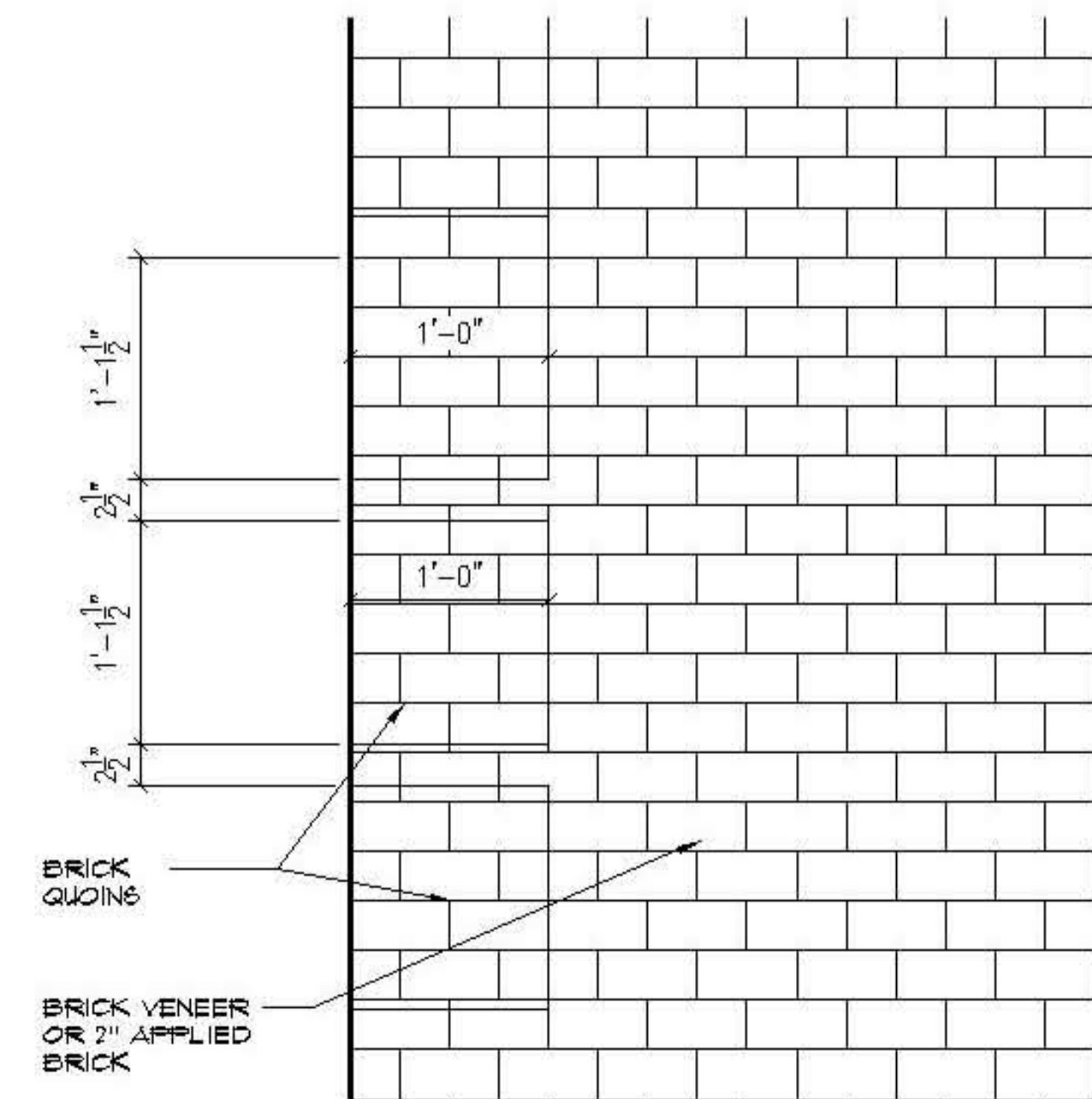
1 A-4 DETAIL BRICK QUOIN SCALE : 1" = 1'-0"
