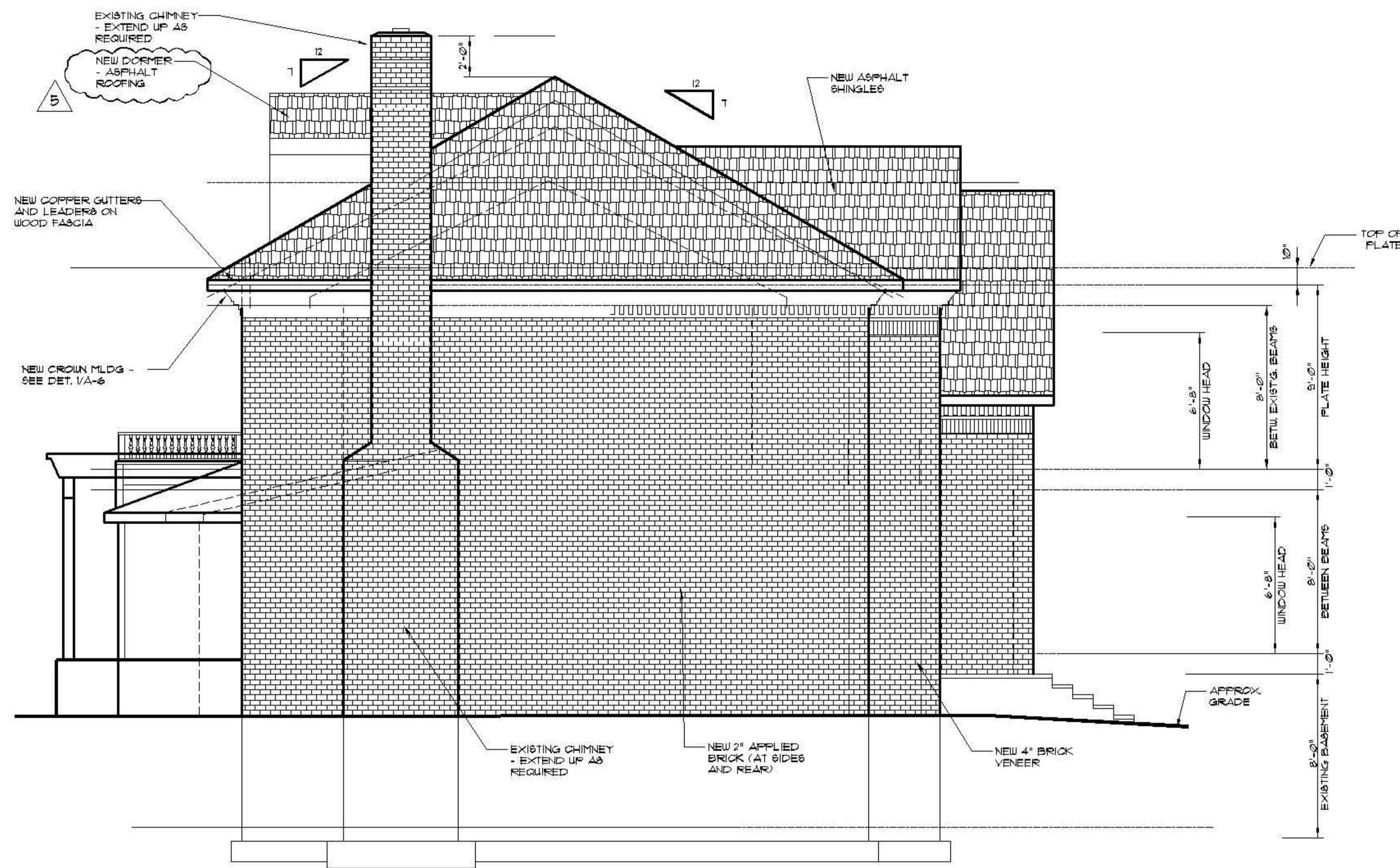
LEFT SIDE ELEVATION
