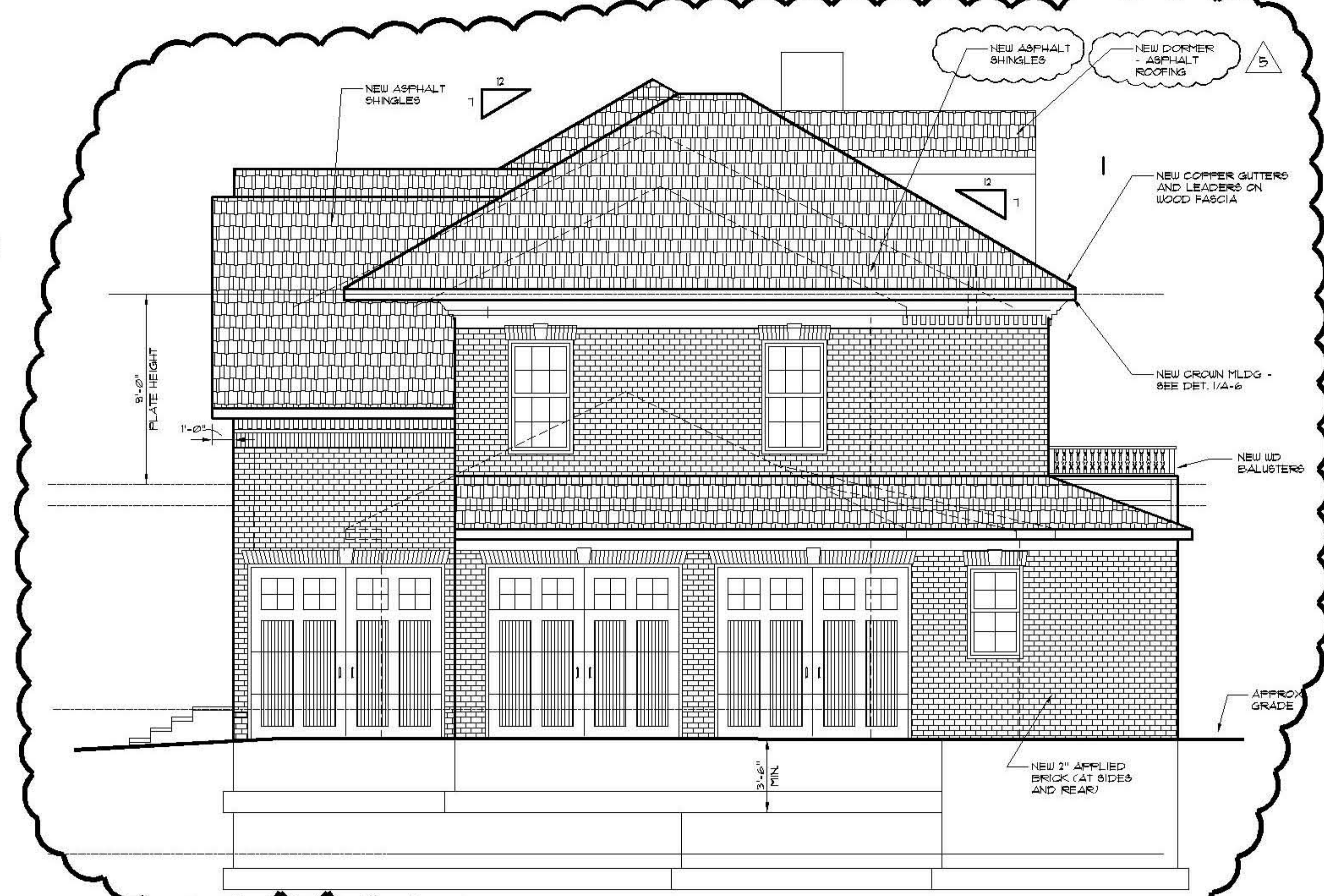
RIGHT SIDE ELEVATION
