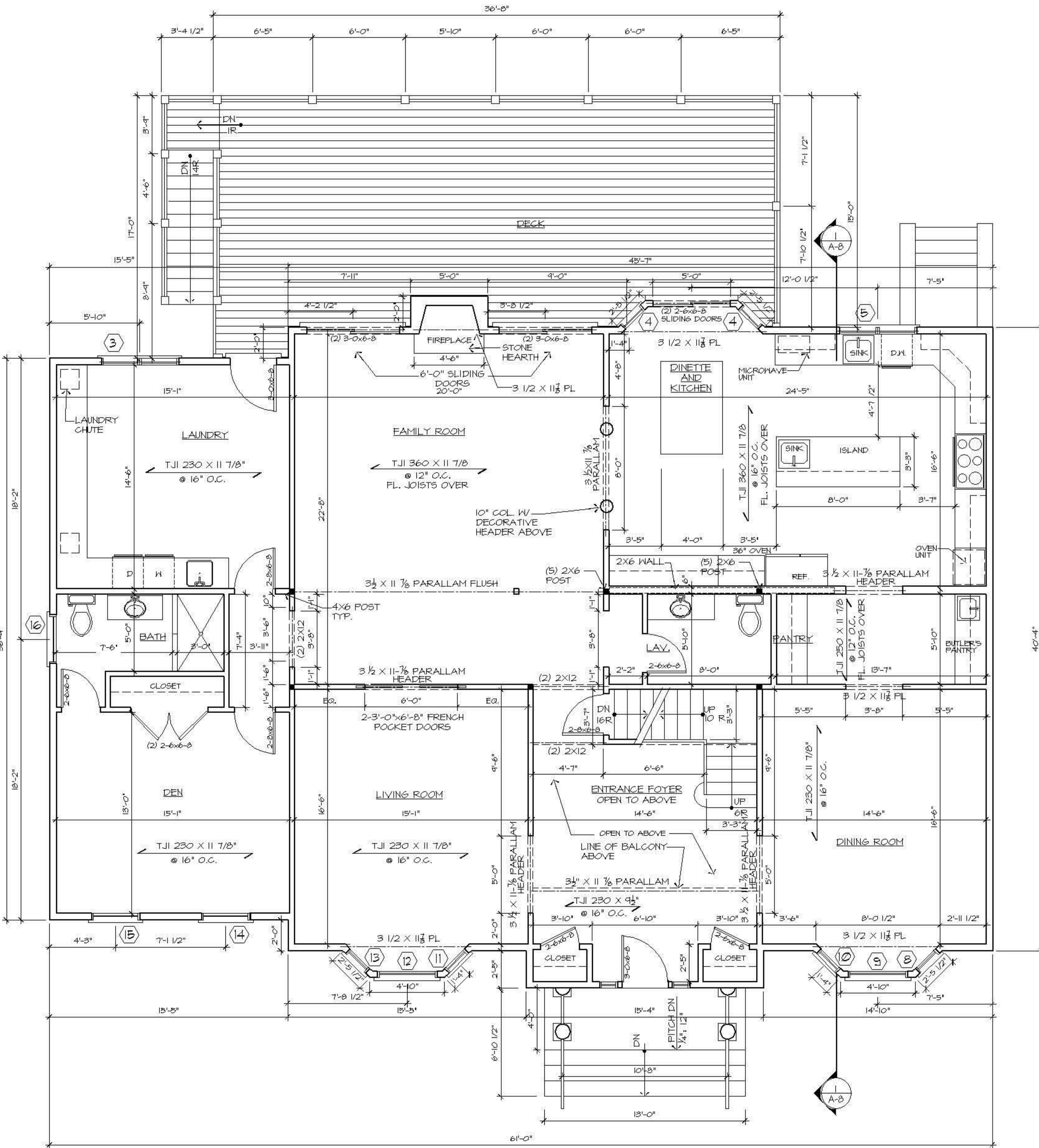
1ST FLOOR PLAN SCALE: 1/4"=1'-0"
