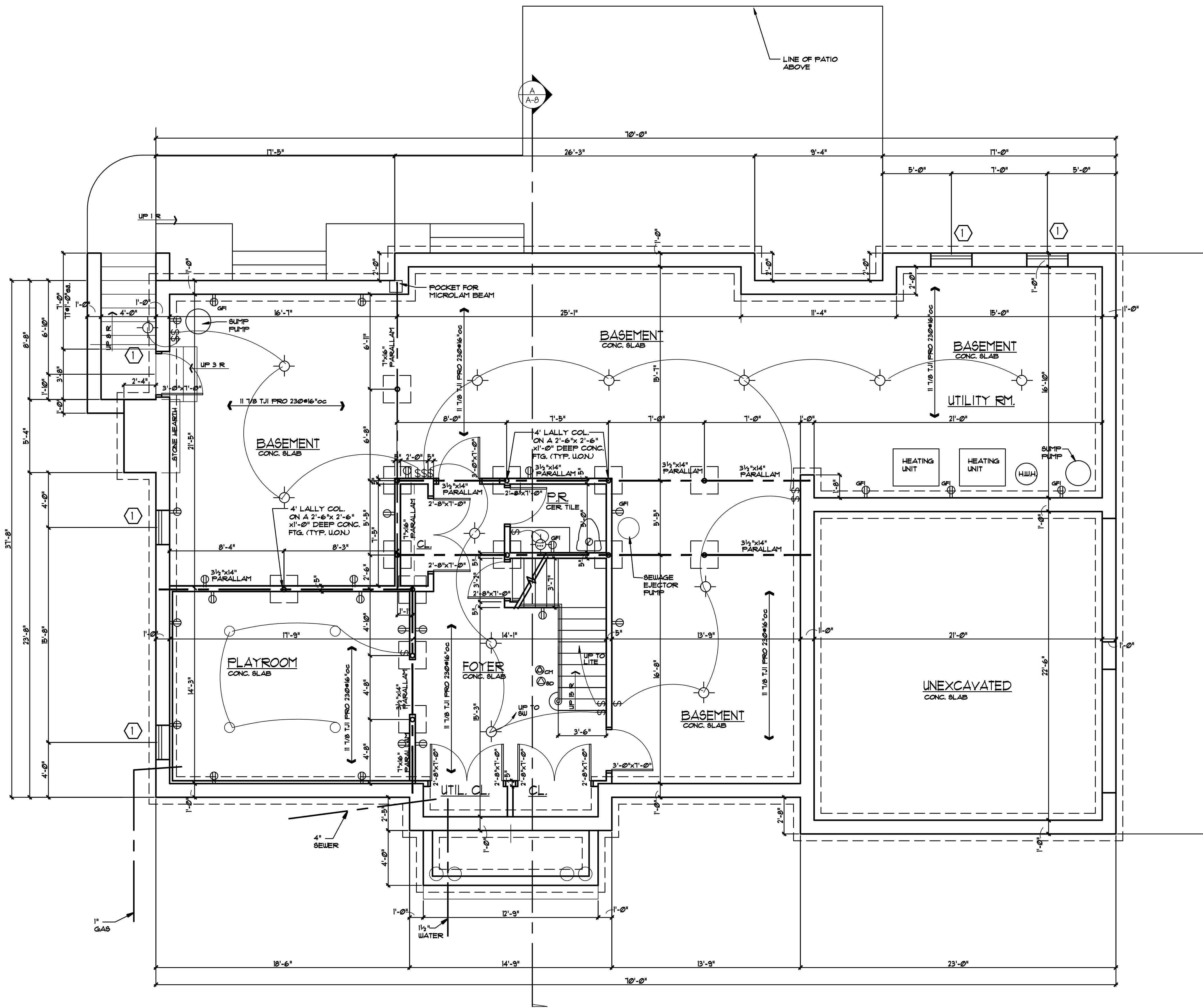
BASEMENT PLAN SCALE: 1/4" = 1'-0"
