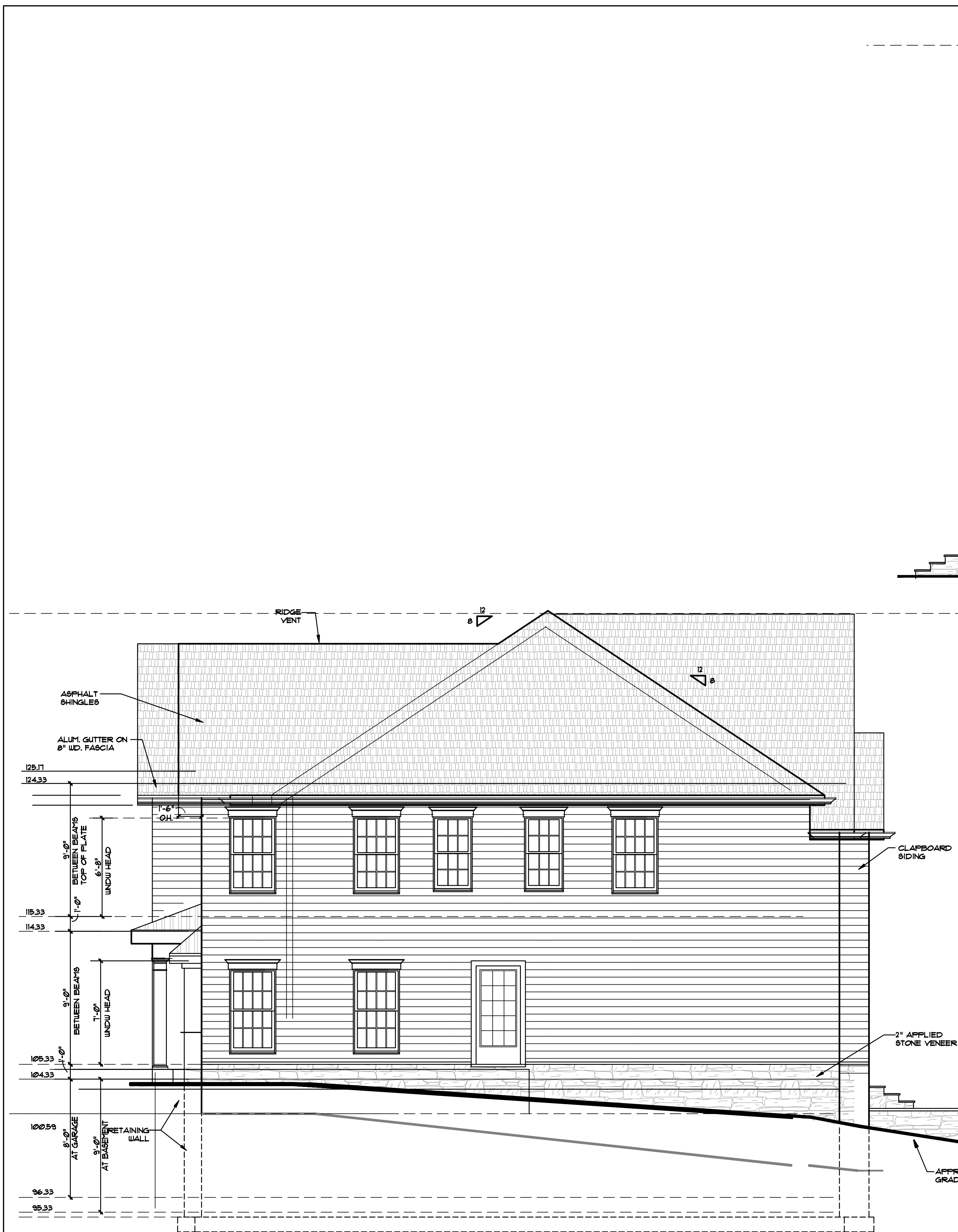
RIGHT SIDE ELEVATION
