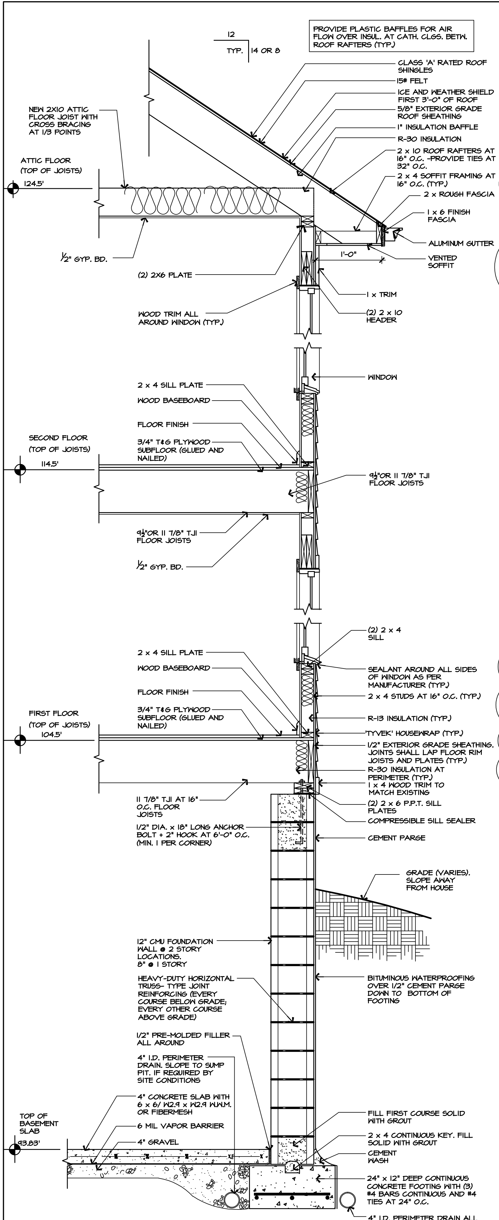
2 TYPICAL WALL SECTION SCALE: 3/4" = 1'-0"
