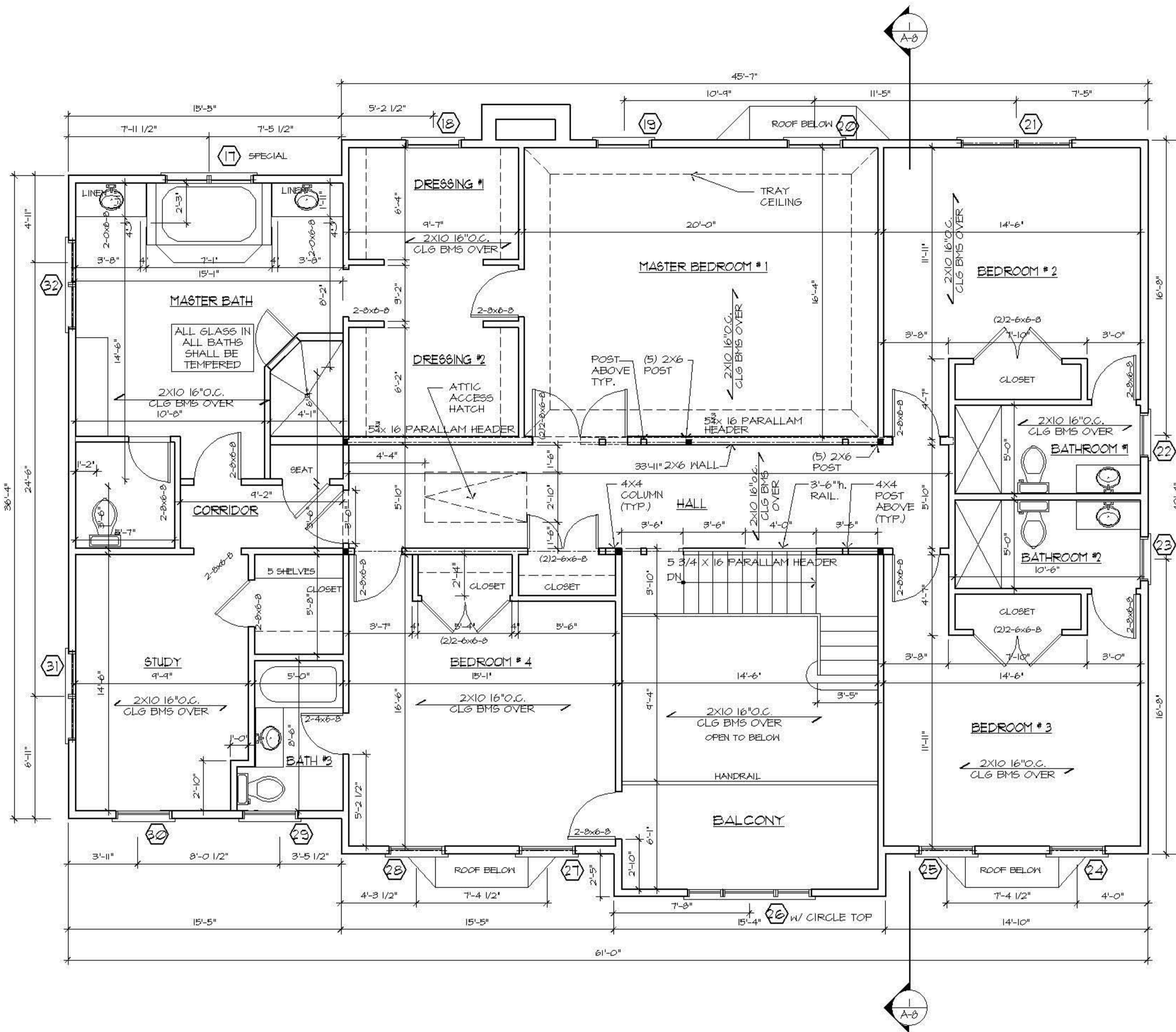
2ND FLOOR PLAN SCALE: 1/4"=1'-0"
