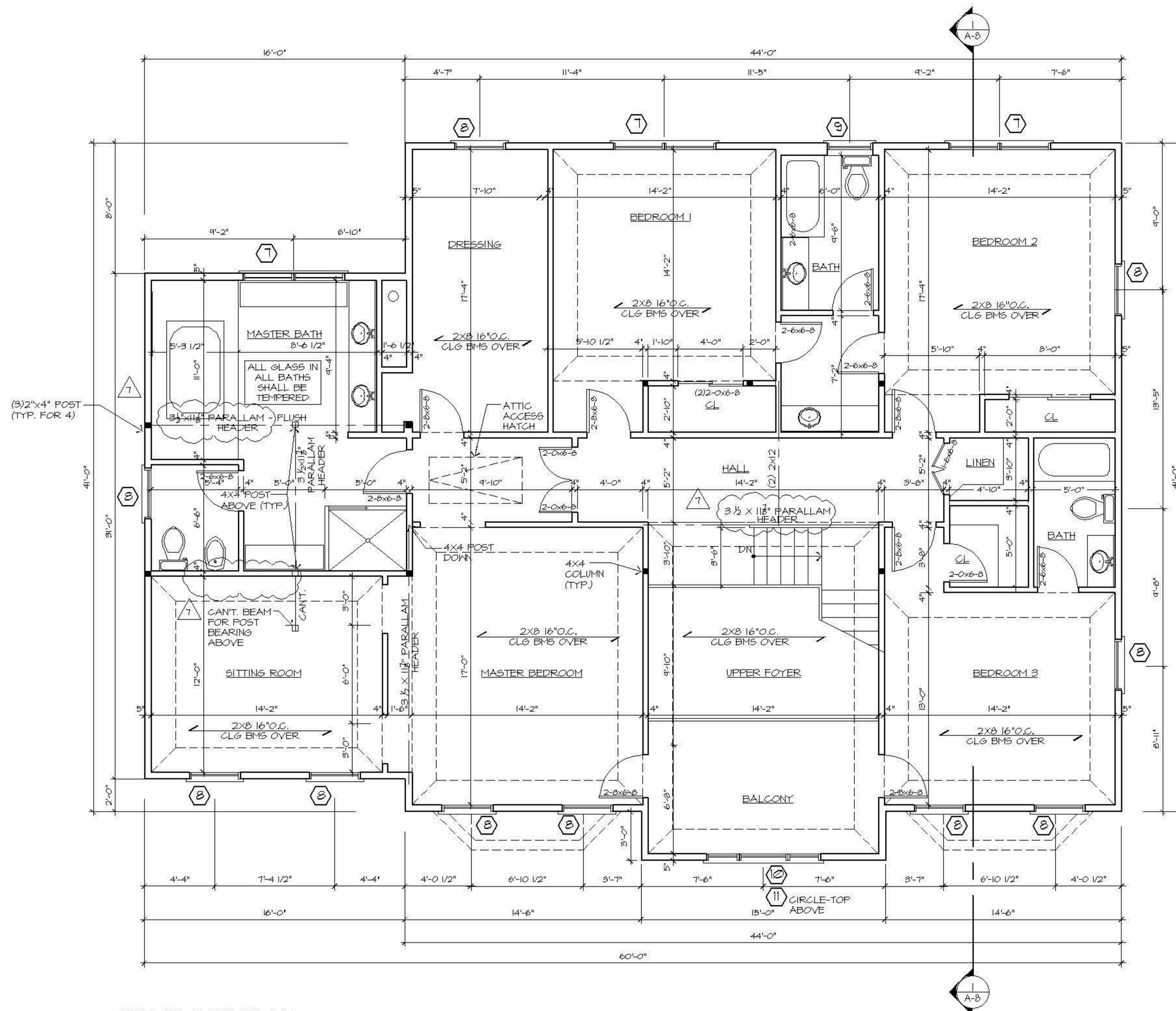
2ND FLOOR PLAN SCALE: 1/4"=1'-0"
